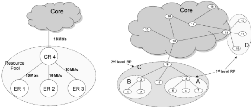
Fig. 4. Resource Pool
